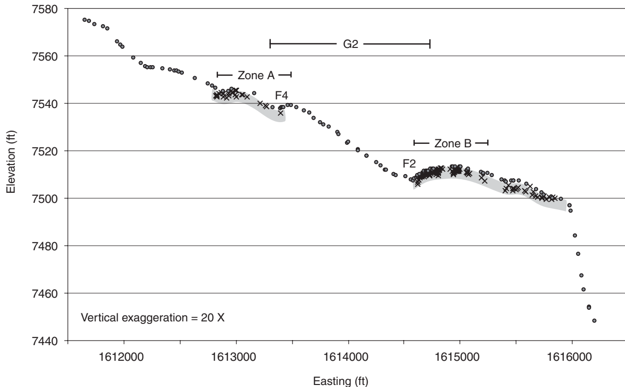
Figure 10. Profile of the TA-9 Trench Showing Surveyed Data. The filled circles are points on the ground surface at the edge of the trench. The X symbols are points at contact between Qbt and post-Qbt strata. Gray bands indicate areas in the trench where Qbt was observed. In all other areas, post-Qbt strata are thicker than the trench depth. Structural features F2, F4, and G2 are as in Plate 1.
